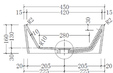
B-B Section
