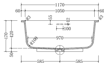
B-B Section
