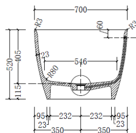
B-B Section
