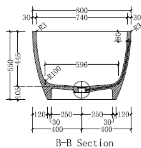
B-B Section
