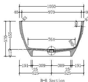
B-B Section
