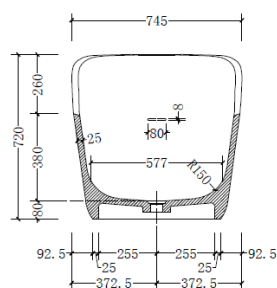
B-B Section
